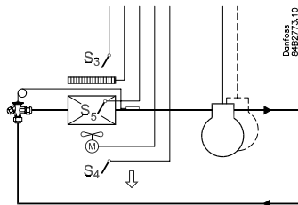
Expansion valve
