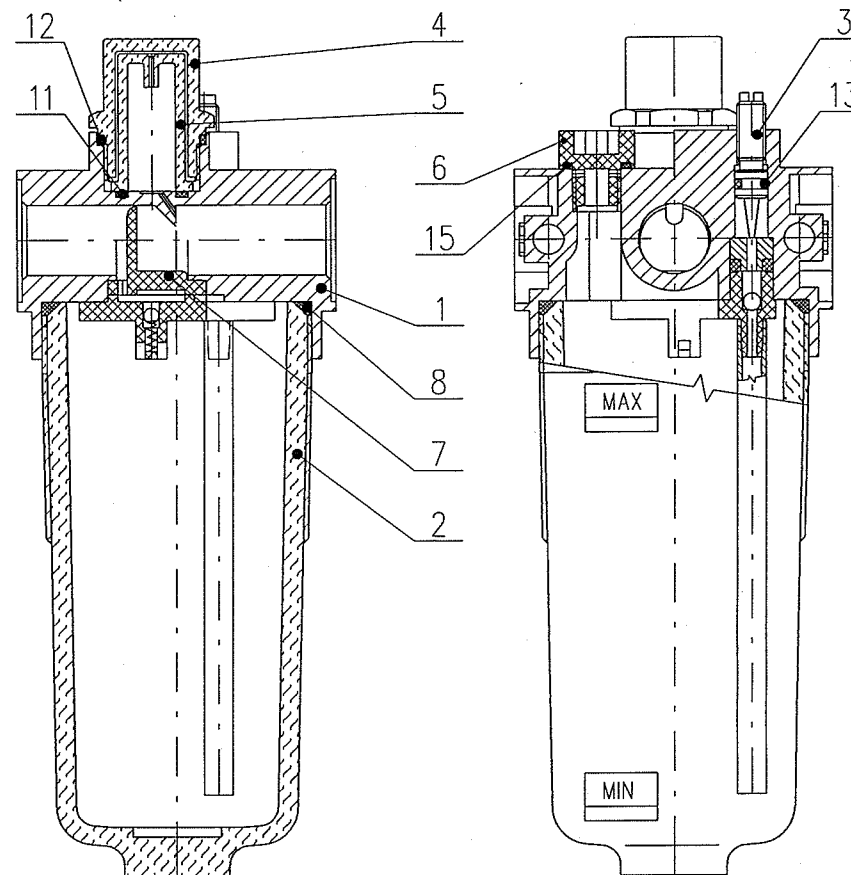
Fig. 1: Lubricators M3/8 and M1/2
