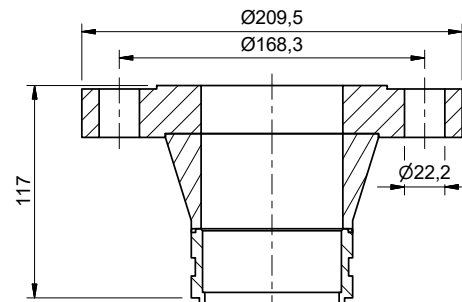
IN80 (3" - 300 Lb)
