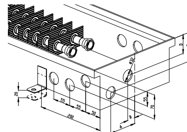
11/28 A=80, B=20, C=74, D=57 11/34 A=79, B=10, C=70, D=62 11/42 A=120, B=31, C=70, D=54
