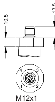
M12x1
