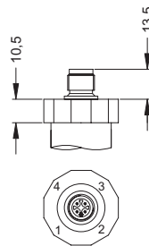
M 12x1
