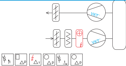
Схема 2.2 VAC-E-ShD1D3D35D125Te
