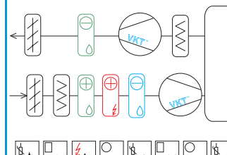
Схема 3.5 VAC-W-ShD1D3D35D35D125Te
