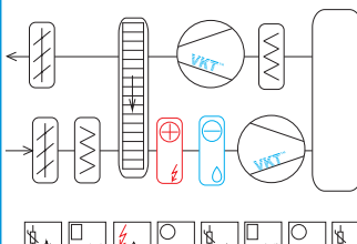
Схема 3.4 VAC-W-ShD1D3D35D35D125Te
