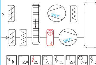
Схема 2.4 VAC-E-ShD1D3D35D35D125Te
