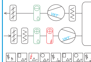
Схема 2.5 VAC-E-ShD1D3D35D35D125Te
