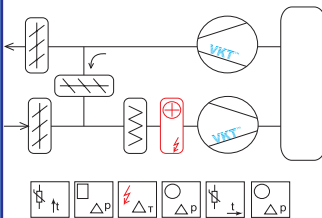
Схема 2.3 VAC-E-ShD1D3D35D125Te
