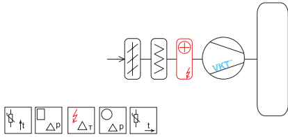
Схема 2.1 VAC-E-ShD1D3D35D125Te
