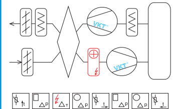
Схема 2.6 VAC-E-ShD1D3D35D35D125Te
