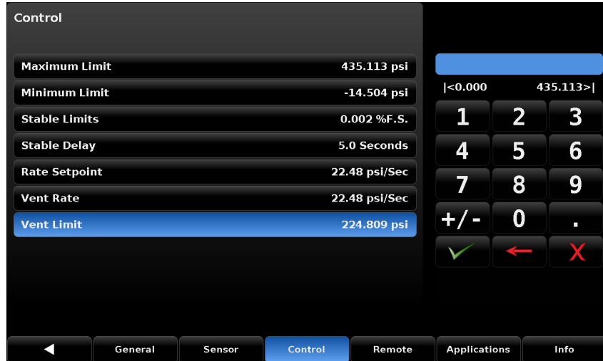
Figure 7.3.5 - Vent Limit
