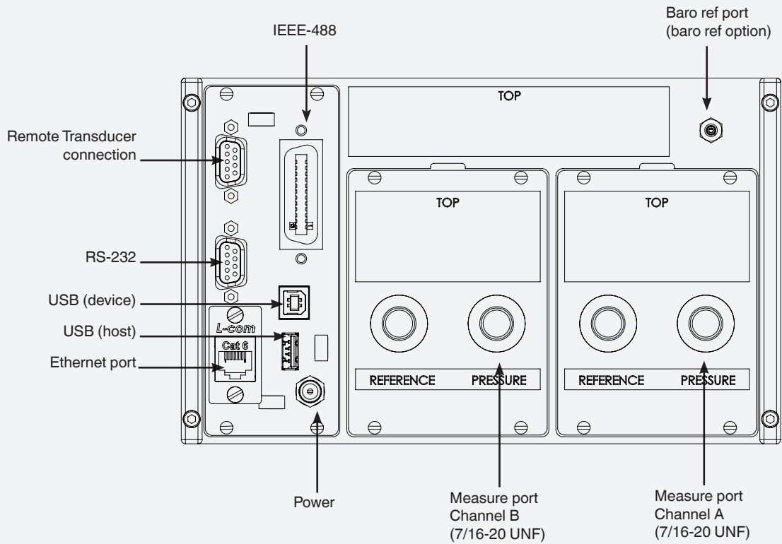
Rear Panel
