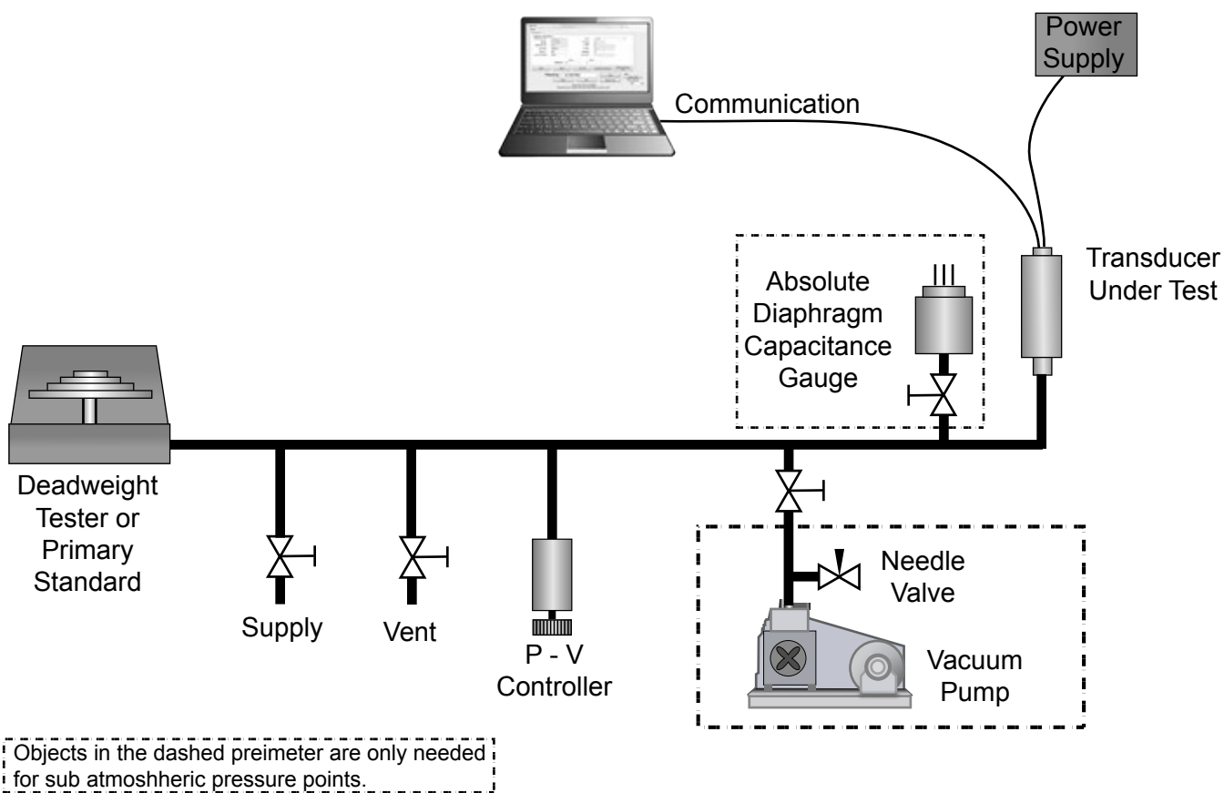
Figure 7.2.5 - Calibration Setup
