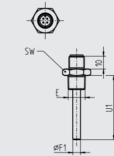
Circular connector M12 x 1
